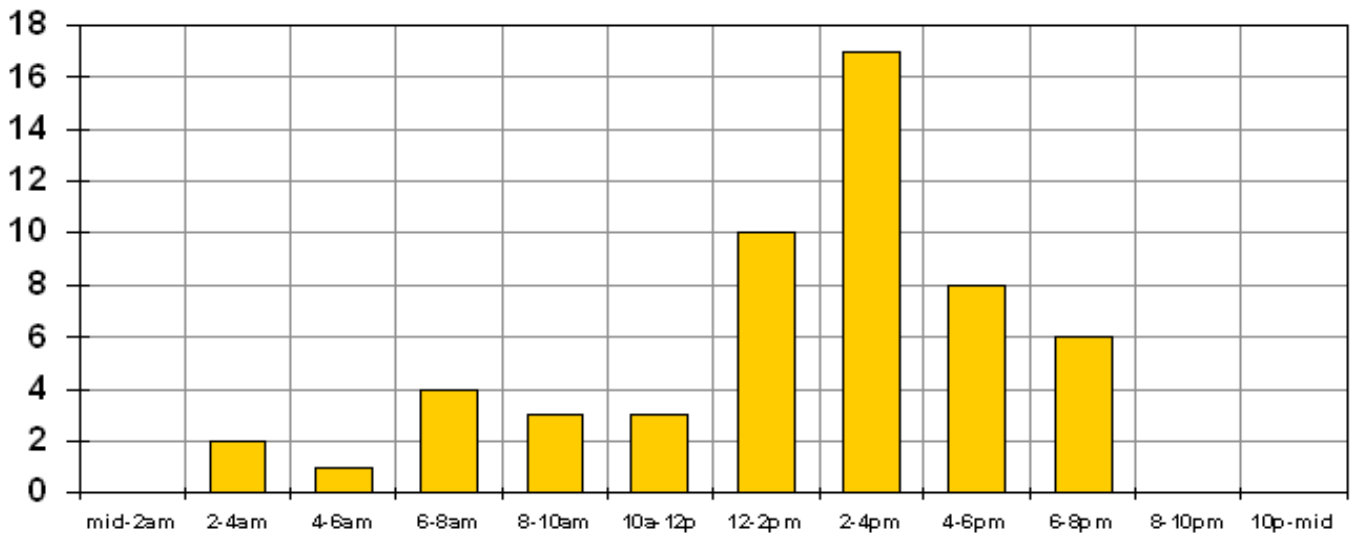
Time of SE TX Lightning Events 1992 - 2008
