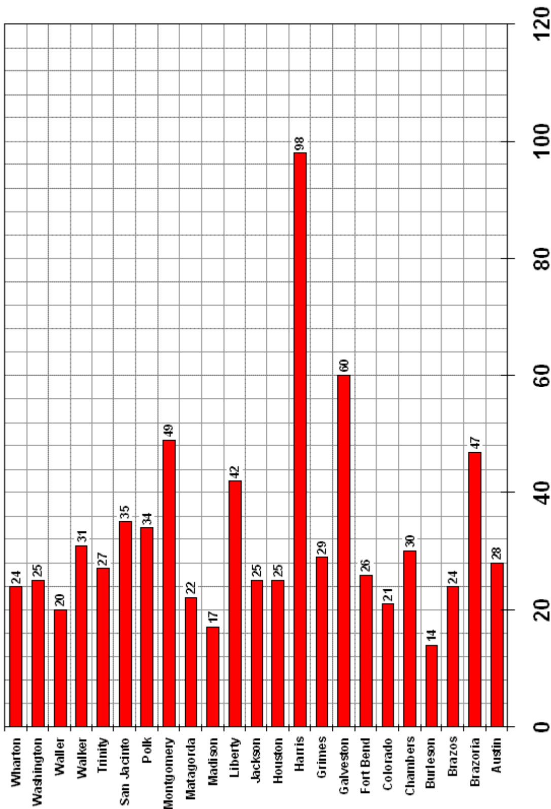
SE Texas Flash Flood Events 1992 - 2008
