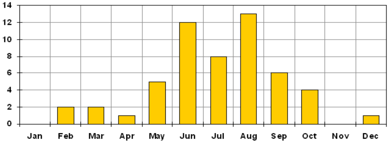
Number of SE TX Lightning Events 1992 - 2008
